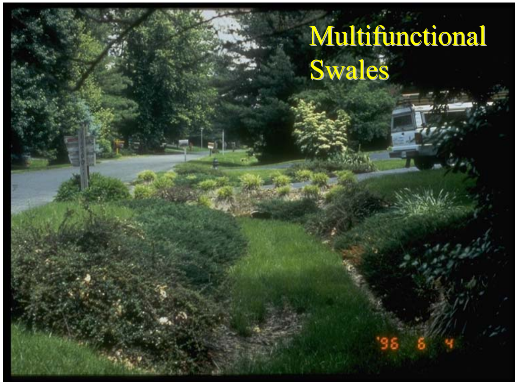
Figure 3-2. Dry Swale
