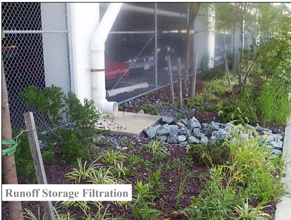
Figure 3-3. Dry Well
